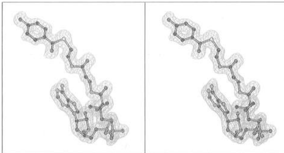
FIGURE 3: Representative electron density. Electron density corresponding to the bound product is shown. The electron density displayed was calculated to 1.8 Å resolution with coefficients of the form (2F_o - F_c) , where F_o and F_c were the native and calculated structure factor amplitudes, respectively. The map was contoured at 1\sigma .
