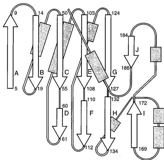
FIGURE 2: Topological diagram for the large domain of the dehalogenase subunit. \beta -Strands are represented as arrows while \alpha -helices are displayed as cylinders. The numbering refers to those amino acid residues at the beginning and end of the \beta -strands.
