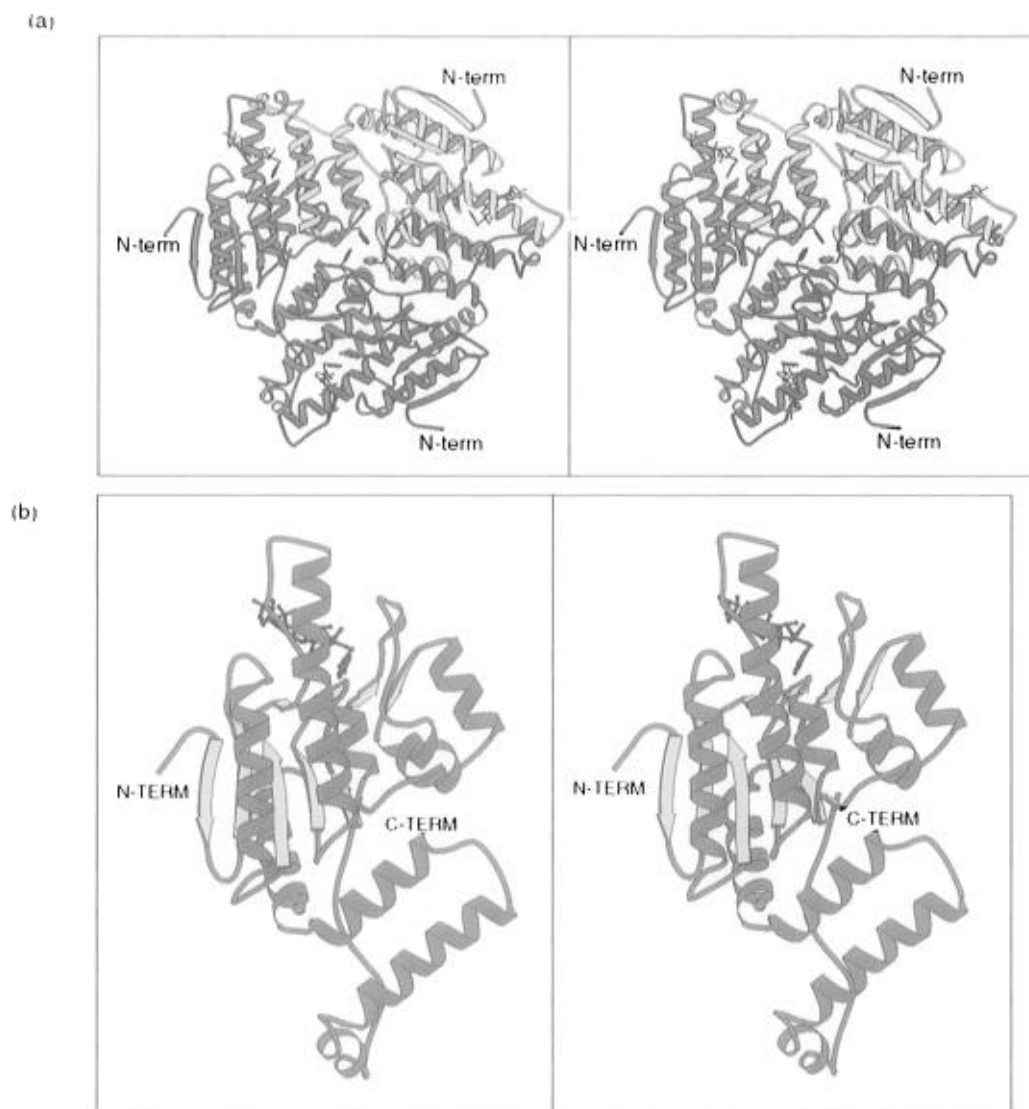
FIGURE 1: Ribbon representations of the 4-chlorobenzoyl-CoA dehalogenase. These figures were prepared with the software package MOLSCRIPT (Kraulis, 1991). (a) Each subunit is displayed in a different color with the bound products, 4-hydroxybenzoyl-CoA, depicted in ball-and-stick representations. (b) Ribbon representation of one subunit of the dehalogenase. The position of the calcium ion connecting the two domains is indicated by the green sphere.
