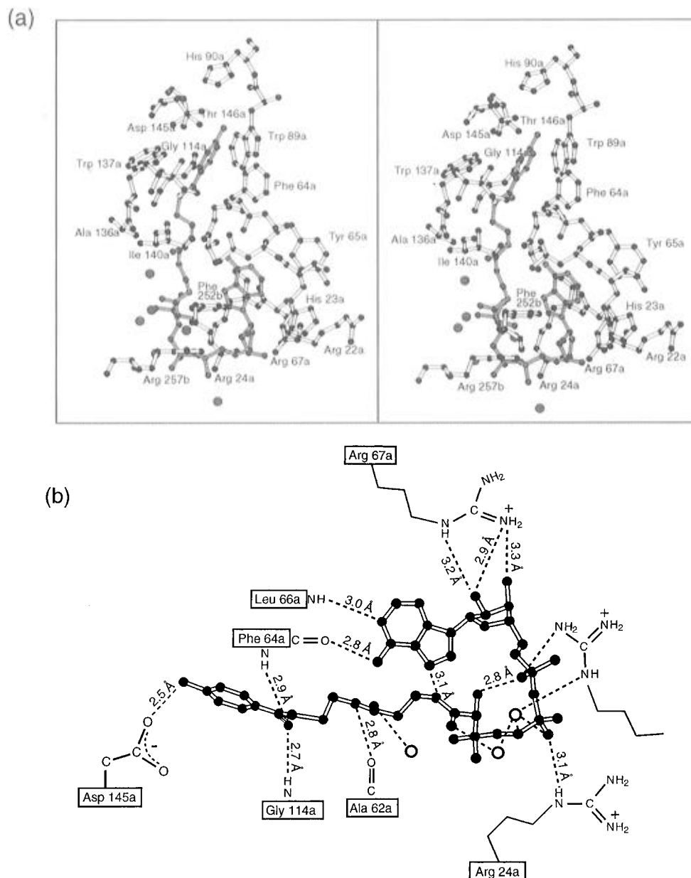
FIGURE 4: Structural features of the active site of the dehalogenase. (a) Close-up view of the active site for subunit I is displayed with those amino acid residues located within approximately 3.8 Å of the 4-hydroxybenzoyl-CoA product. (b) Schematic representation of the electrostatic interactions between the protein and the product in subunit I are indicated by the dashed lines. Those residues with the suffix "b" are contributed by subunit II in the trimer. The bond lengths indicated are average values observed for the three subunits constituting the trimer. Due to crystal packing, the protein/product interactions in the vicinity of the pantothenate and pyrophosphate moieties are slightly different in subunits II and III. Water molecules are indicated by the open circles.
